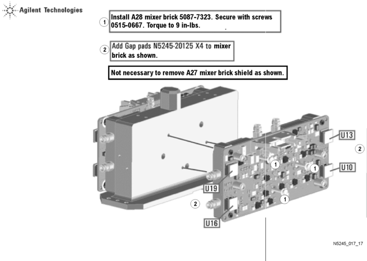
Figure 1 A28 Mixer Brick Assembly
