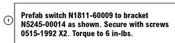
Figure 6 A52 Port 4 Mechanical Switch Assembly
